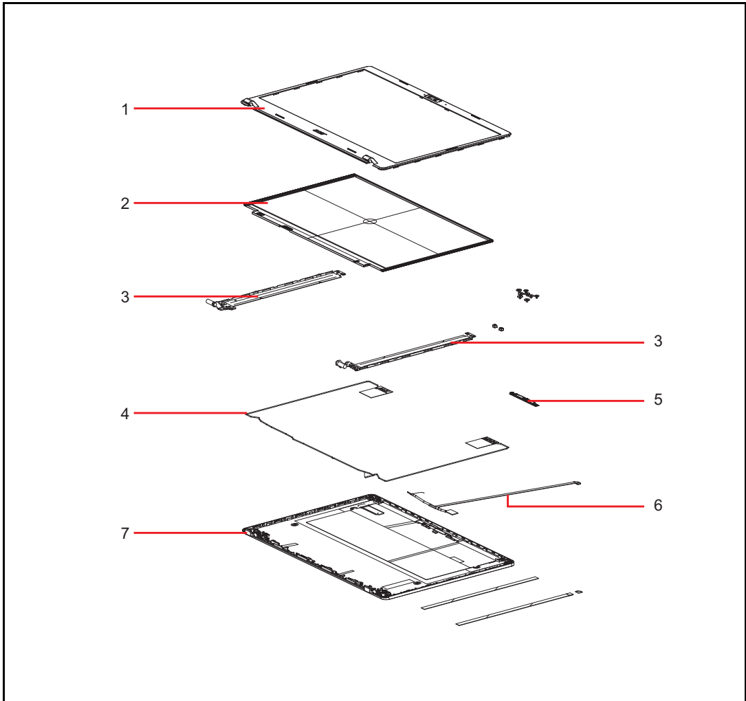
Figure 1-60. LCD Assembly Exploded Diagram
