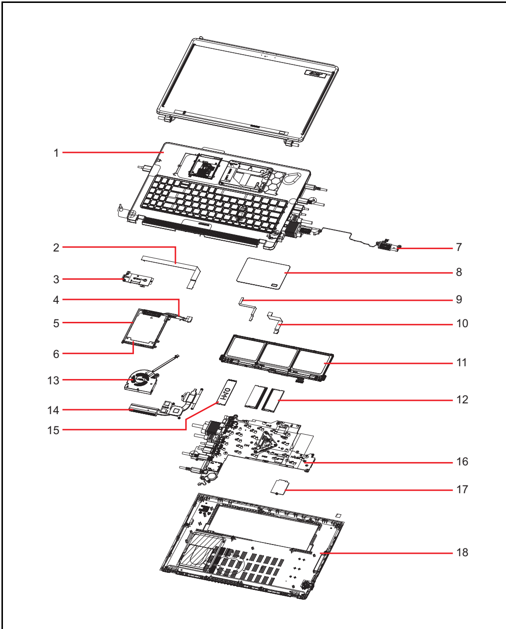
Figure 1-59. System Exploded Diagram
