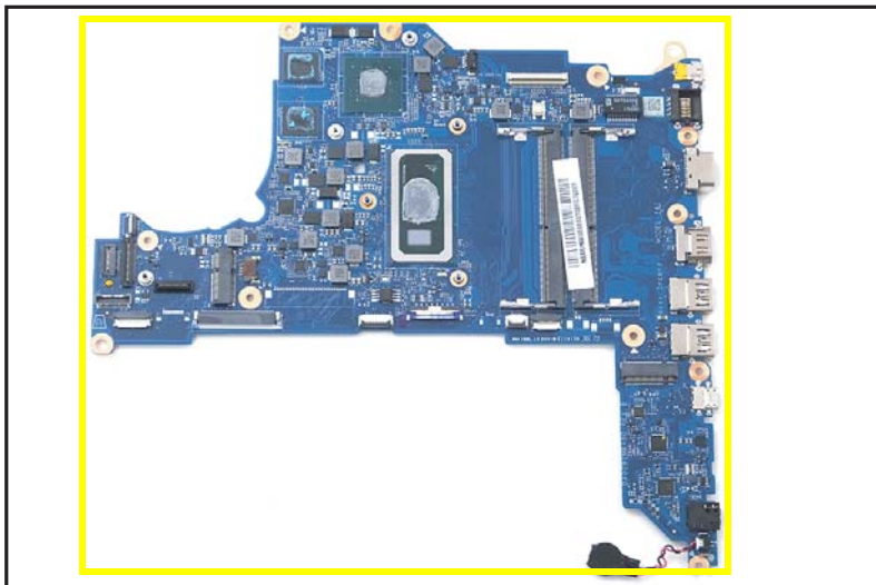
Figure 1-48. Mainboard
